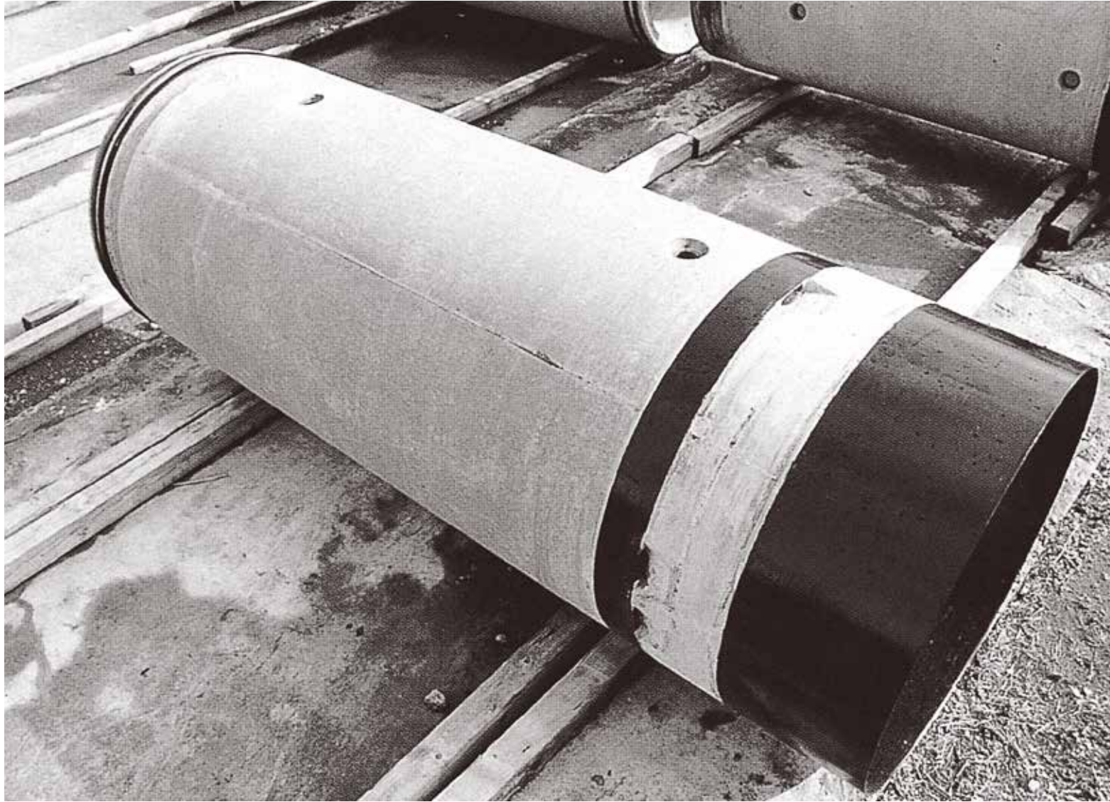
Jacking Pipe for Lubricant Injection [Type A]
